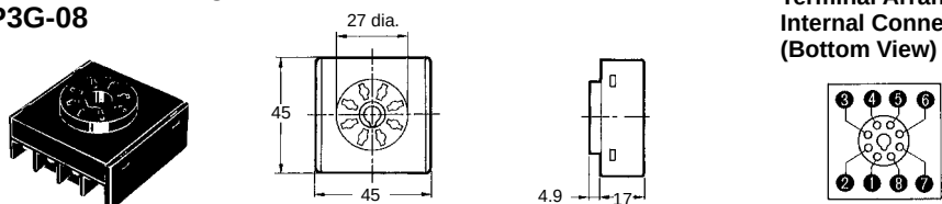
Terminal Arrangement/ Internal Connections (Bottom View)
