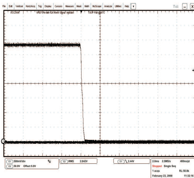
Figure 14. Power Off Waveform
