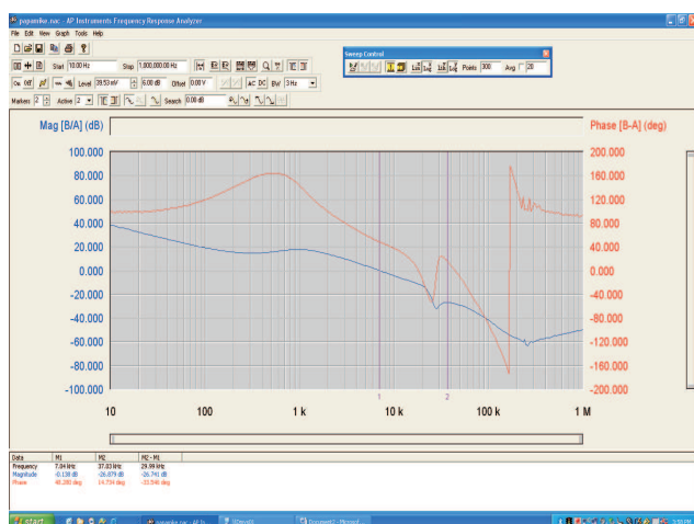
Figure 5. Loop Response Gain and Phase 36 V in 0-A Load
