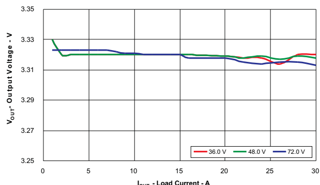
Figure 4. Line and Load Regulation
