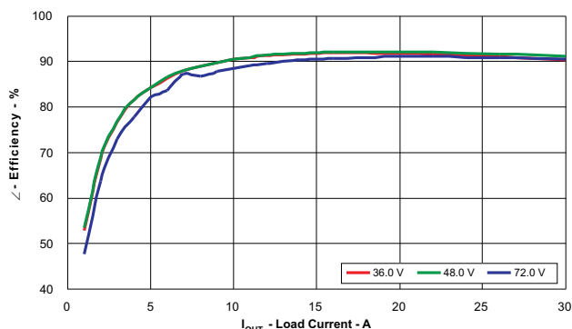
Figure 3. UCC2897A-EVM Efficiency
