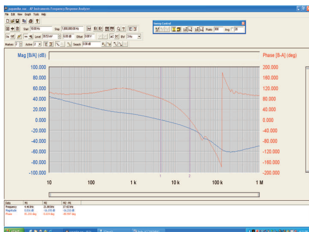
Figure 7. Loop Response Gain and Phase 72 V in 30-A Load
