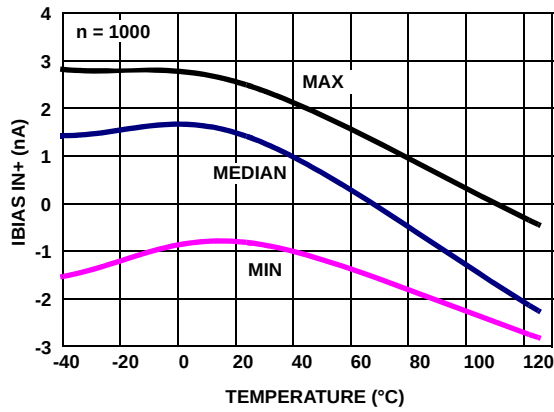
FIGURE 25. I_{\text{BIAS IN}+} vs TEMPERATURE, V_+ , V_- = \pm 2.5V
