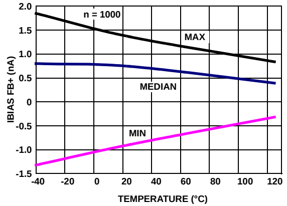
FIGURE 26. I_{\text{BIAS FB}+} vs TEMPERATURE, V_+ , V_- = \pm 2.5V
