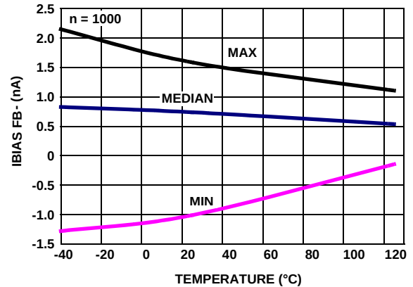
FIGURE 28. I_{\text{BIAS FB}-} vs TEMPERATURE, V_+ , V_- = \pm 2.5V
