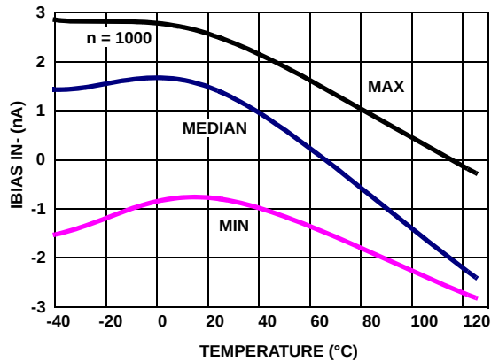
FIGURE 27. I_{\text{BIAS IN}-} vs TEMPERATURE, V_+ , V_- = \pm 2.5V
