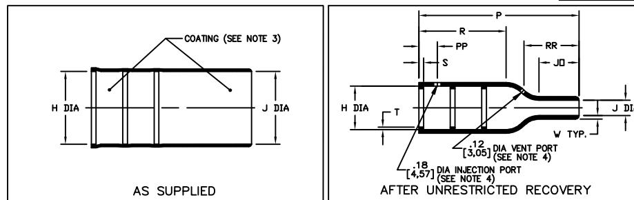
PART NUMBER H J P ±10% b R Ref b S Ref b T Ref b JO ±10% b W ±20% b PP ±10% b RR ±10% b Min Max Min -3,-4, -6,-8,-25 a Min -5,-12, -100 a Max a b a b a 202D121 .92 [23,3] .41 [10,5] .92 [23,3] .49 [12,4] .22 [5,6] 1.50 [38,1] .83 [21,1] .12 [3,0] .04 [1,0] .40 [10,2] .07 [1,78] .60 [15,2] N/A 202D132 1.12 [28,4] .56 [14,3] 1.12 [28,4] .58 [14,7] .26 [6,6] 2.16 [54,9] 1.09 [27,7] .12 [3,0] .04 [1,0] .65 [16,5] .07 [1,78] .60 [15,2] .85 [21,6] 202D142 1.22 [31,0] .70 [17,8] 1.22 [31,0] .63 [16,0] .28 [7,2] 2.63 [66,8] 1.39 [35,3] .12 [3,0] .04 [1,0] .70 [17,8] .08 [2,03] .60 [15,2] .96 [24,5] 202D153 1.42 [36,0] .88 [22,4] 1.42 [36,0] .73 [18,5] .33 [8,4] 3.15 [80,0] 1.63 [41,4] .12 [3,0] .04 [1,0] .82 [20,8] .08 [2,03] .60 [15,2] 1.17 [29,7] 202D163 1.68 [42,7] 1.11 [28,2] 1.68 [42,7] .87 [22,0] .39 [9,9] 4.08 [103,6] 2.22 [56,4] .12 [3,0] .065 [1,65] .97 [24,9] .09 [2,29] .60 [15,2] 1.44 [36,7] 202D174 2.04 [51,8] 1.38 [35,1] 2.04 [51,8] 1.39 [35,3] .62 [15,8] 5.13 [130,3] 2.54 [64,5] .12 [3,0] .065 [1,65] 1.56 [39,6] .13 [3,3] .60 [15,2] 2.12 [53,8] 202D185 2.60 [66,0] 1.75 [44,5] 2.60 [66,0] 1.80 [45,7] .80 [20,4] 6.50 [165,1] 3.31 [84,1] .12 [3,0] .08 [2,0] 1.90 [48,3] .16 [4,06] .60 [15,2] 2.59 [65,6] 202D196 3.22 [81,7] 2.27 [57,6] 3.22 [81,7] 2.25 [57,1] 1.00 [25,4] 7.00 [177,8] 3.75 [95,3] .12 [3,0] .08 [2,0] 1.88 [47,8] .16 [4,06] .60 [15,2] 2.64 [67,1]
