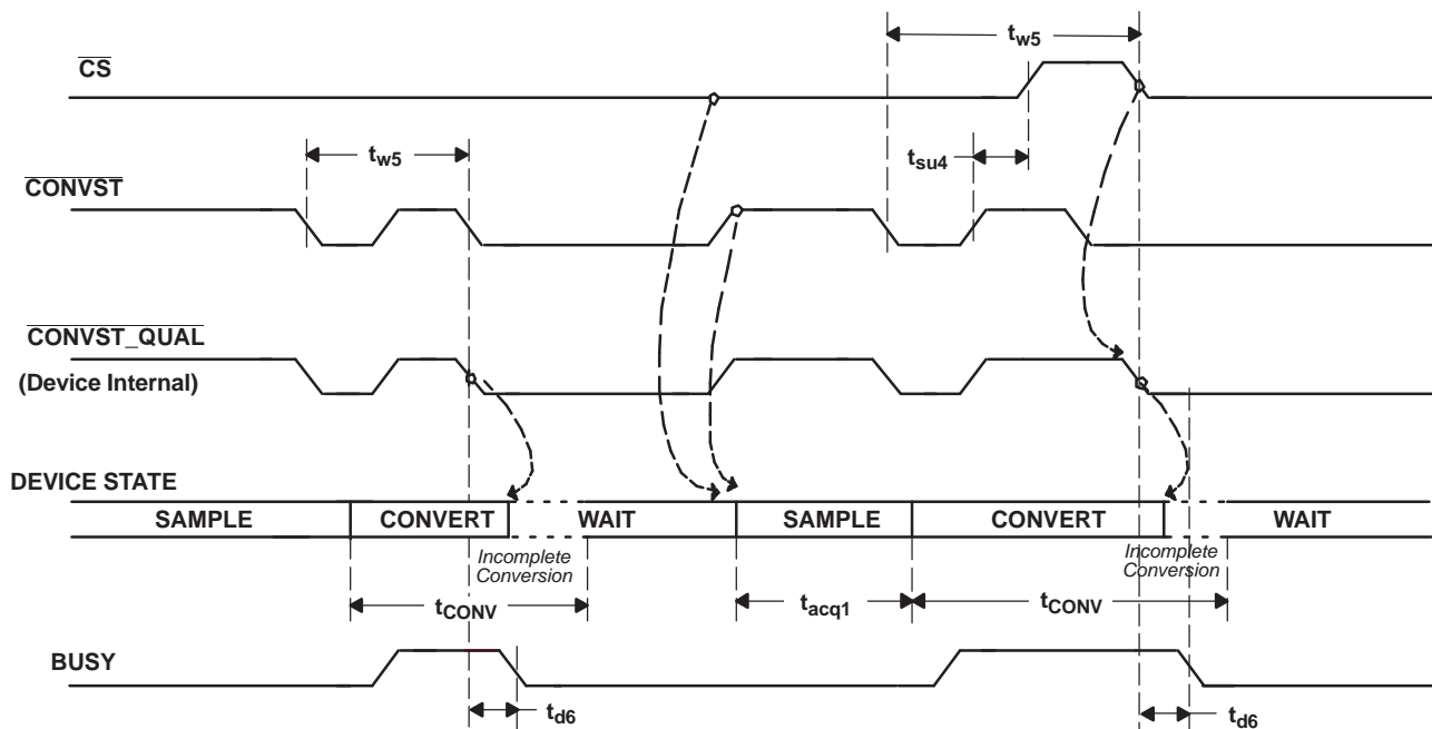
Figure 44. Conversion Abort
