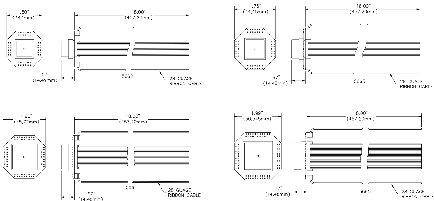
PLCC SOCKET ADAPTER CABLE CHART
