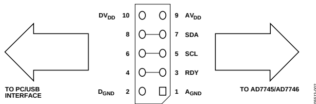
Figure 3. LK2 10-Pin (2 × 5) Header
