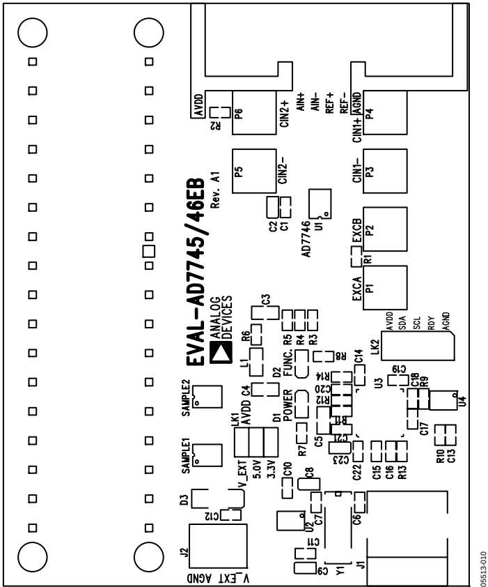
Figure 11. AD7746 Evaluation Board Layout
