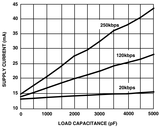
FIGURE 9. SUPPLY CURRENT vs LOAD CAPACITANCE WHEN TRANSMITTING DATA
