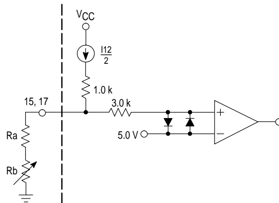
Figure 4. FH Switches
