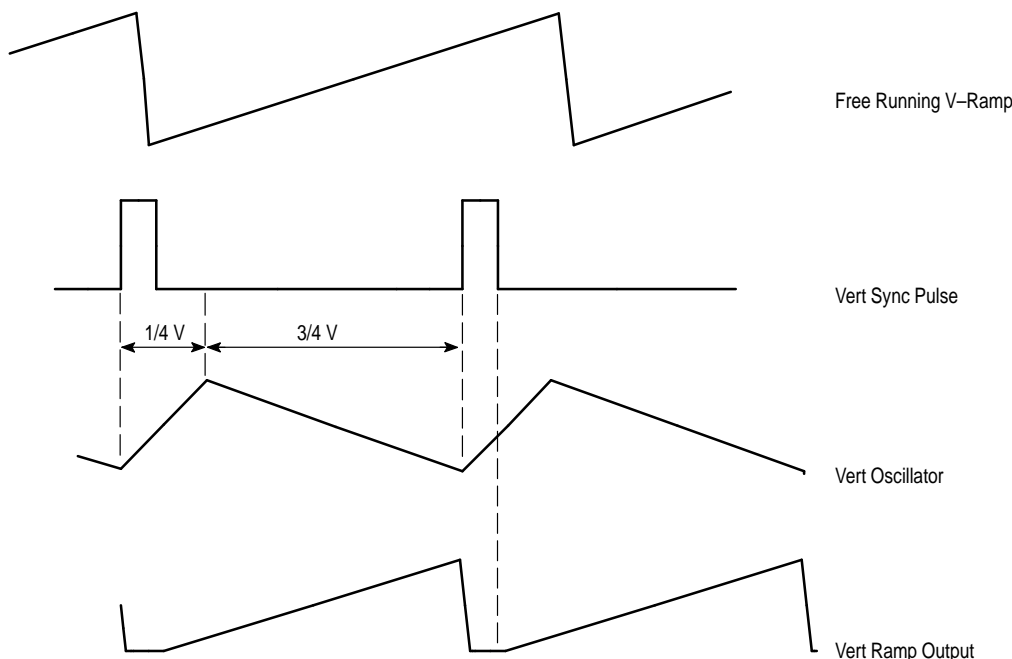
Figure 10. Vertical Section
