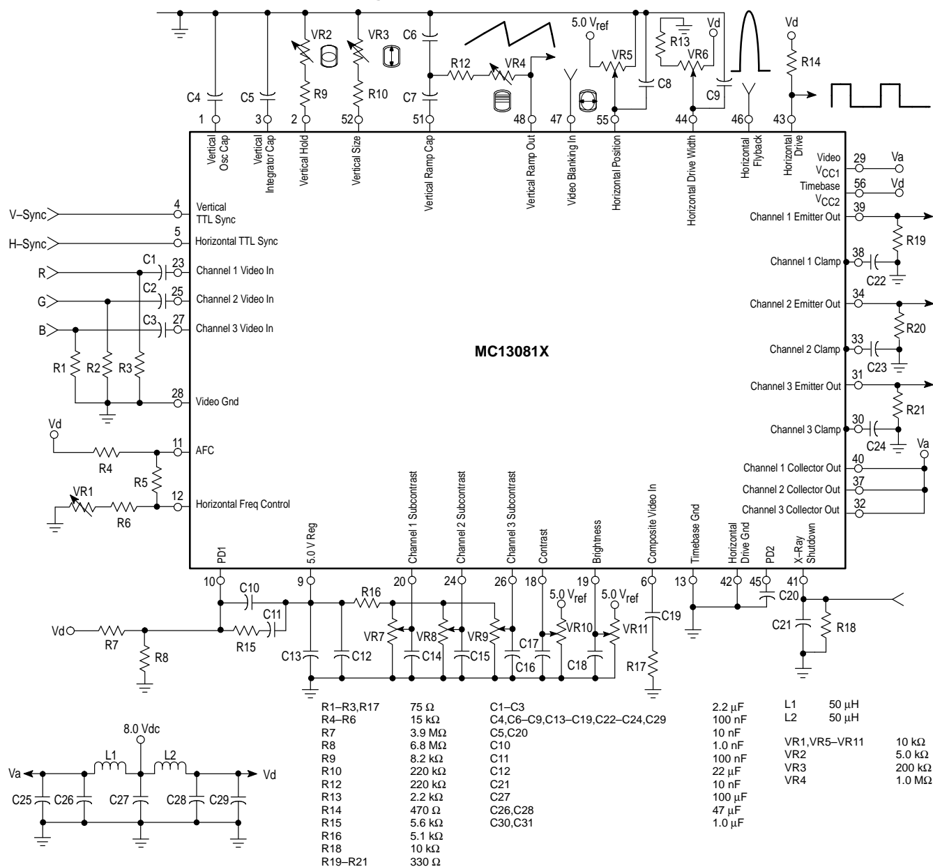
Figure 2. Application Circuit
