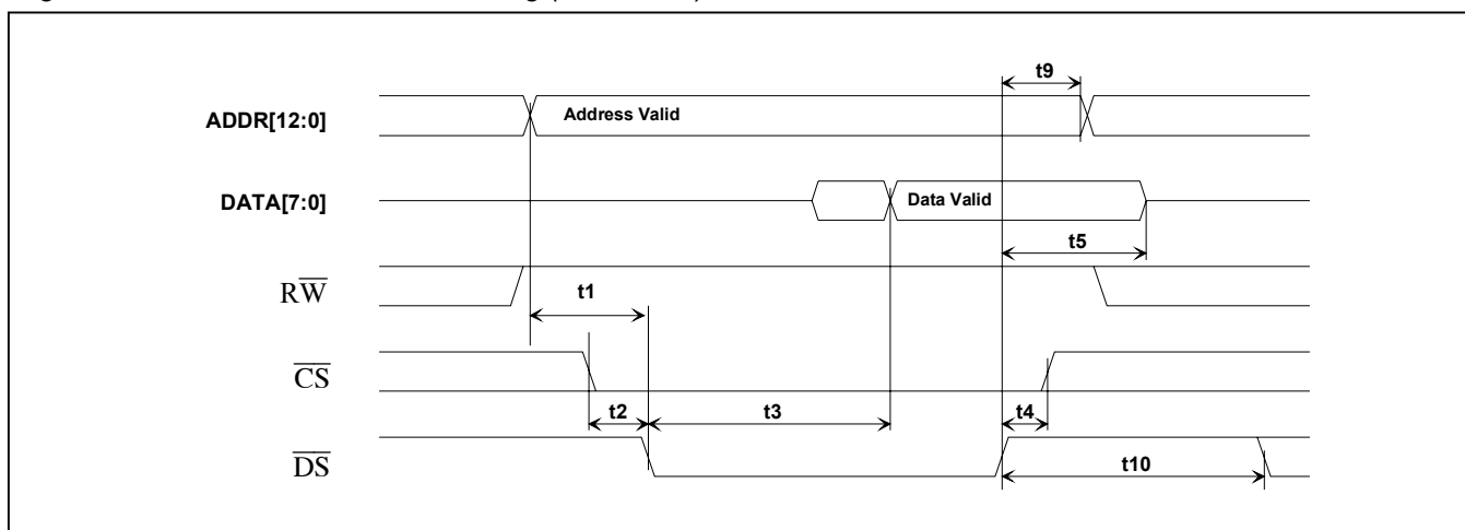
Figure 12-15. Motorola Bus Read Timing (MODE = 1)
