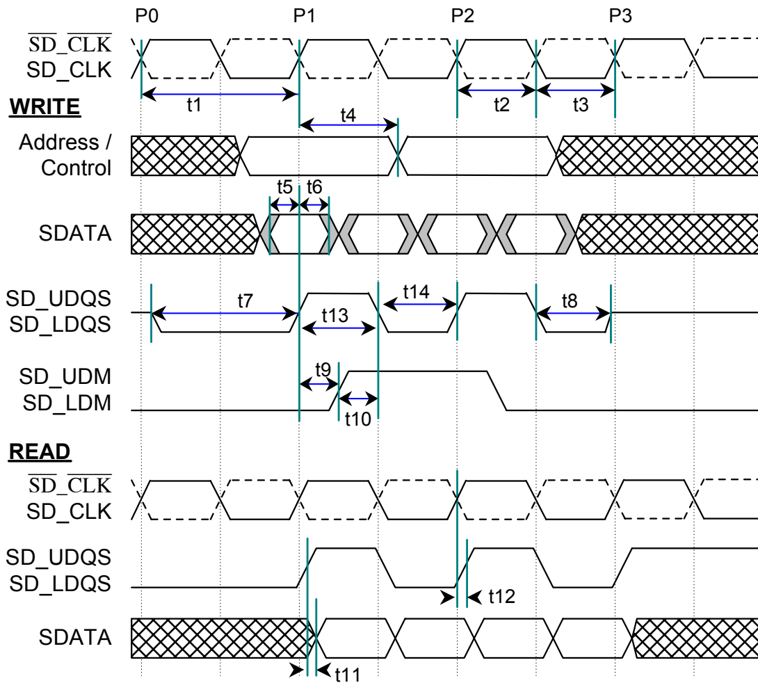
Figure 12-12. DDR SDRAM Interface Timing
