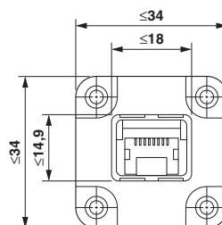
Panel mounting frame dimensional drawing
