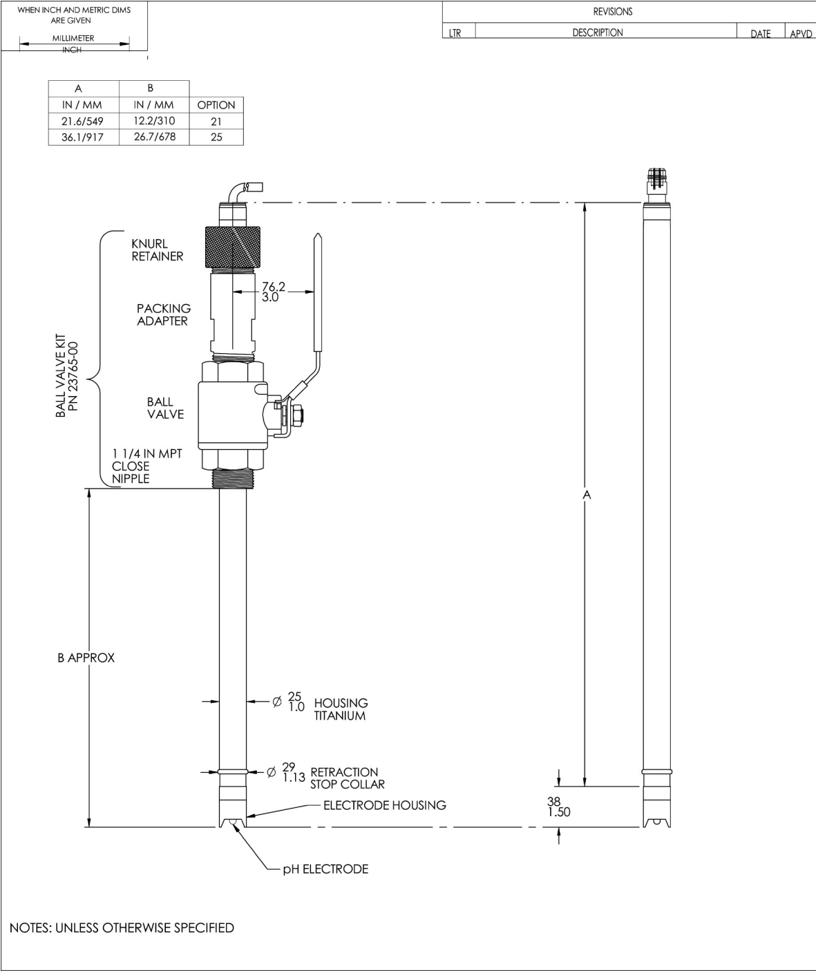
Dimensional Drawing – 3400HT with 1 1/4" Ball Valve Kit PN 23765-00 Note: Add five (5) inches to dimension A if mounting a sensor head junction box onto the sensor.
