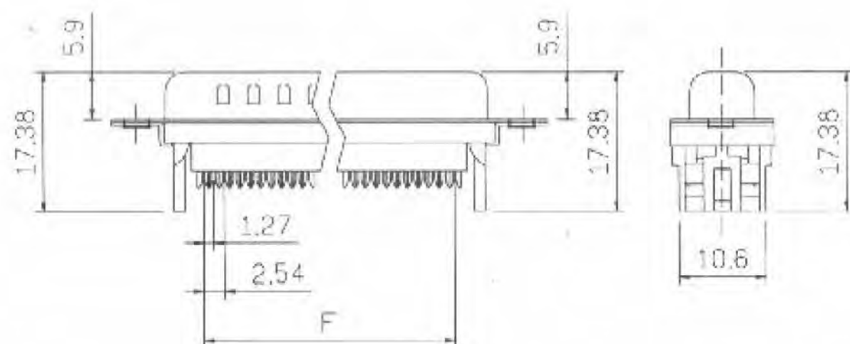
Without Insulator Support
