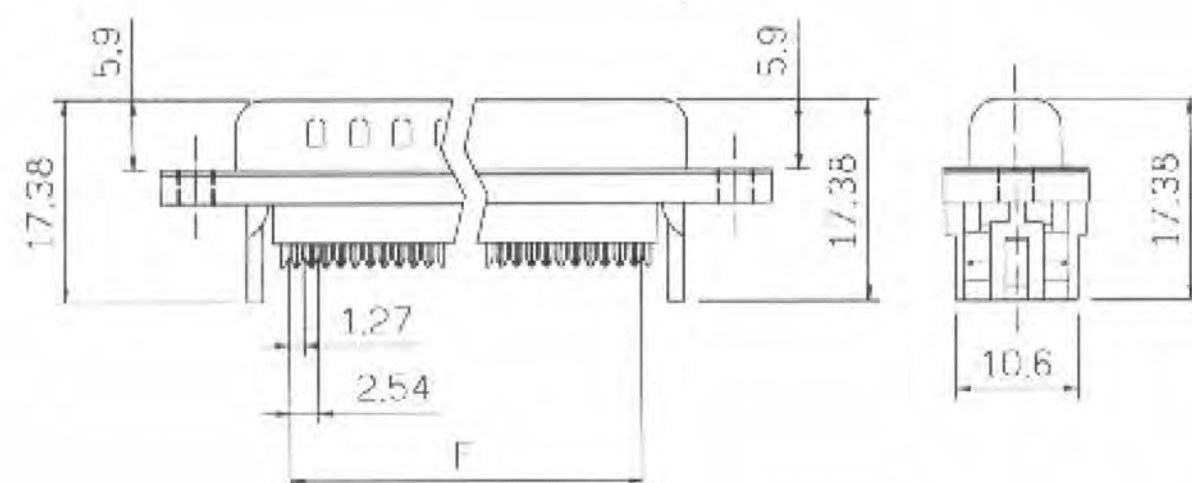
With Insulator Support
