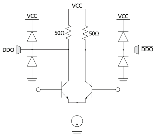
Figure 3-5: High-speed Outputs ( \overline{\text{DDO1/RCO}} , DDO1/RCO, \overline{\text{DDO0}} , DDO0)
