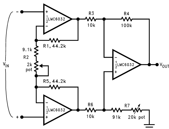
Figure 6-6. Instrumentation Amplifier
