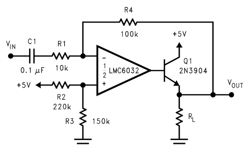
Figure 6-11. Power Amplifier
