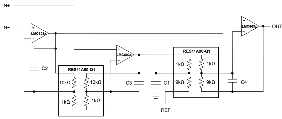
Figure 6-7. Improved Instrumentation Amplifier With RES11A
