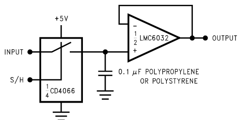
Figure 6-9. Low-Leakage Sample-and-Hold
