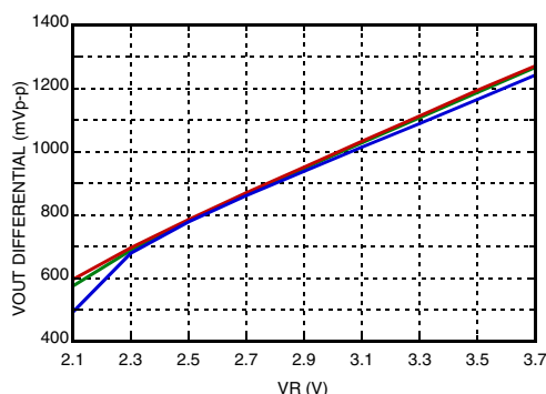
Output Differential Voltage vs. VR [1] [2]
