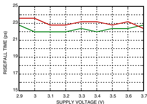
Rise / Fall Time vs. Supply Voltage [1] [2]
