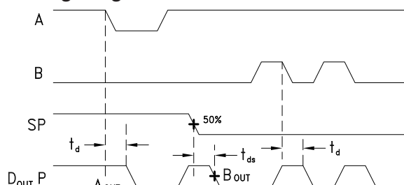
Timing Diagram
