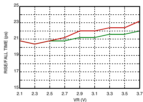
Rise / Fall Time vs. VR [1] [2]
