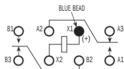
TERMINAL VIEW
