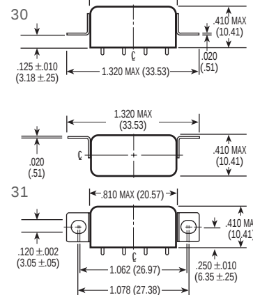
MOUNTING STYLES
