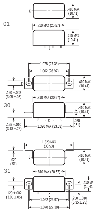
MOUNTING STYLES
