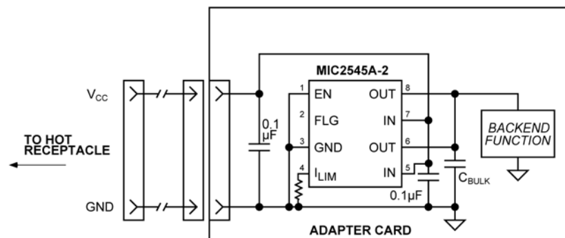
Figure 5. Hot-Plug Application
