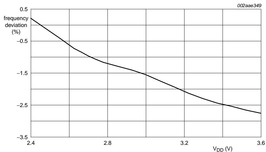
Fig 38. Average watchdog oscillator frequency vs. V_{DD} at -40 °C
