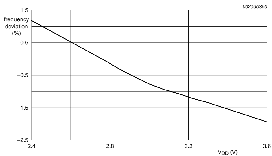
Fig 39. Average watchdog oscillator frequency vs. V_{DD} at +85 °C
