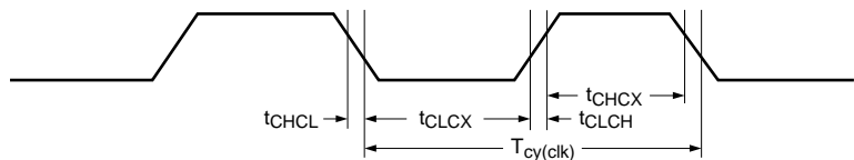
Fig 41. External clock timing (with an amplitude of at least V_{i(RMS)} = 200 mV)
