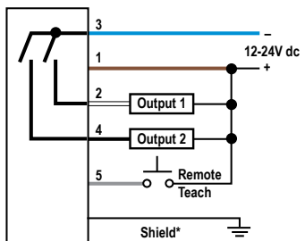
Figure 11. Cabled NPN
