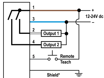
Figure 12. Cabled PNP
