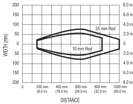
Figure 9. 1-Meter Models
