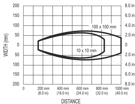
Figure 7. 1-Meter Models
