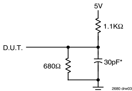
Figure 1. Output Load
