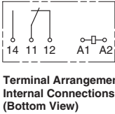
Input circuit
