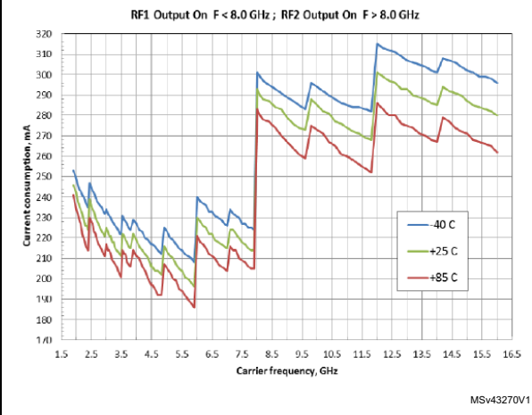
Figure 20. Overall current consumption vs. temperature (3.6 V supply, F_{\text{PFD}}=50 MHz)
