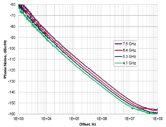
Figure 3. VCO open loop phase noise (5 V supply)
