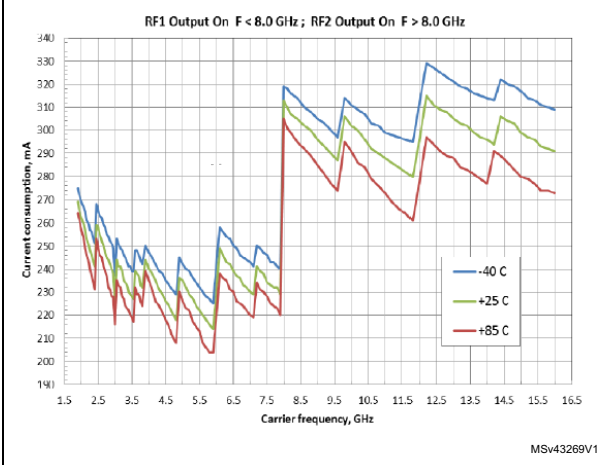
Figure 19. Overall current consumption vs. temperature (5.0 V supply, F_{\text{PFD}}=50 MHz)
