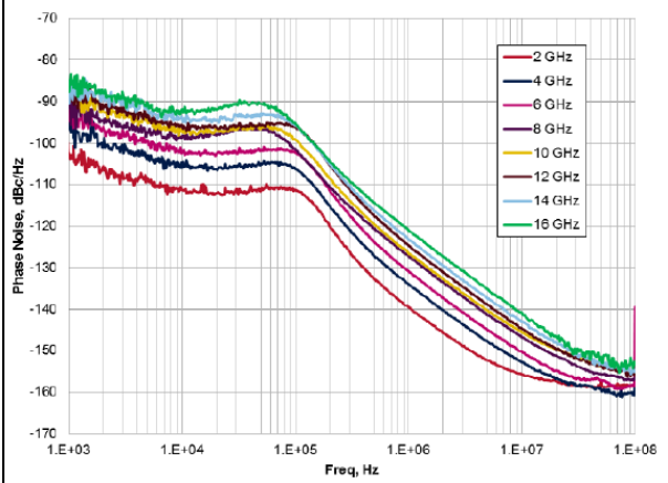
Figure 4. Closed loop phase noise (5 V supply)
