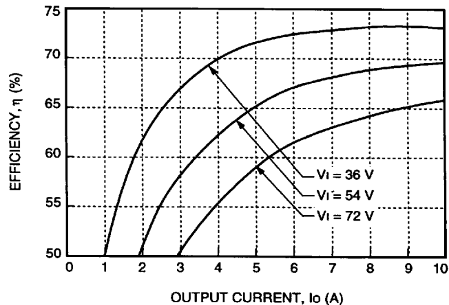
Figure 3. Typical FW050D Efficiency vs. Output Current at Room Temperature
