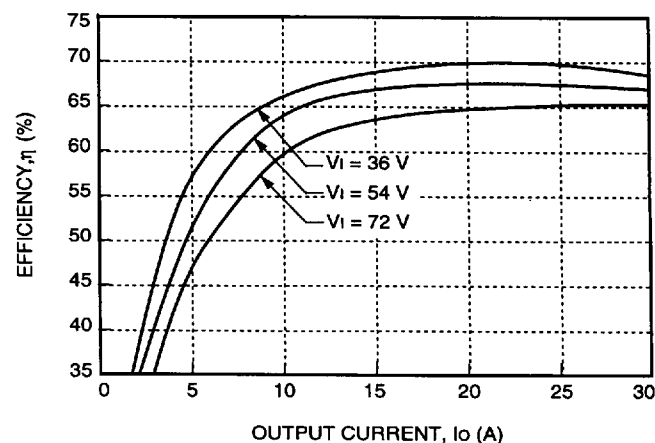
Figure 4. Typical FW150D Efficiency vs. Output Current at Room Temperature
