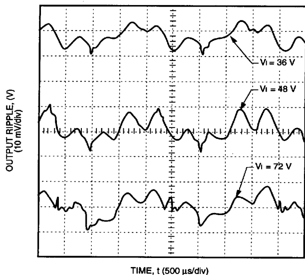
Figure 5. Typical FW150D Output Ripple Voltage at Room Temperature and 30 A Output
