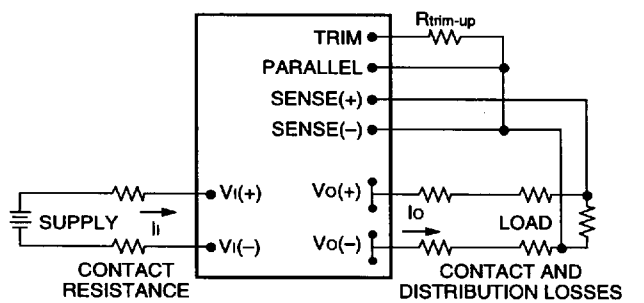
Figure 14. Circuit Configuration to Trim Up Output Voltage
