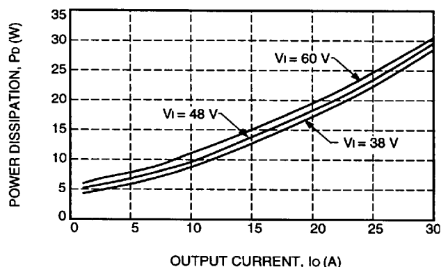
Figure 22. Power Dissipation as Heat vs. Output Current
