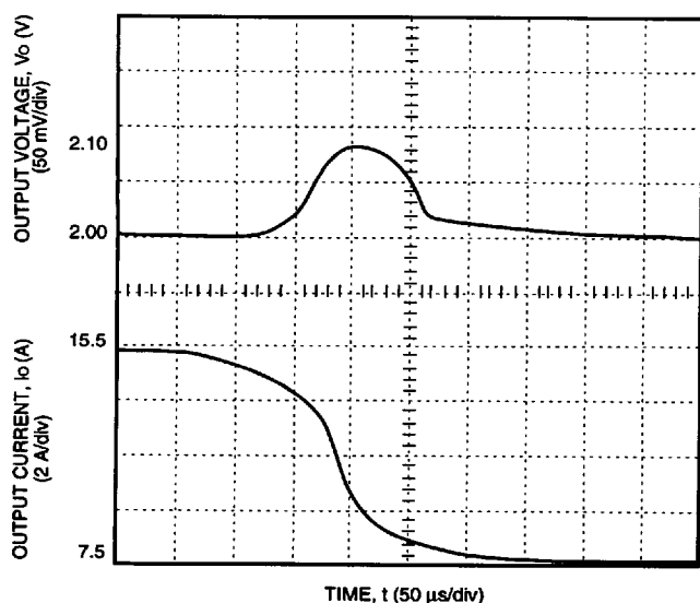
Figure 6. Typical FW150D Transient Response to Step Decrease in Load from 50% to 25% of Full Load at Room Temperature and 48 V Input (Waveform Averaged to Eliminate Ripple Component.)
