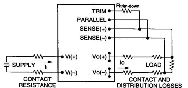
Figure 15. Circuit Configuration to Trim Down Output Voltage
