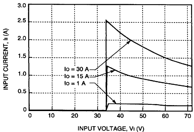
Figure 1. Typical FW150D Input Characteristics at Room Temperature
