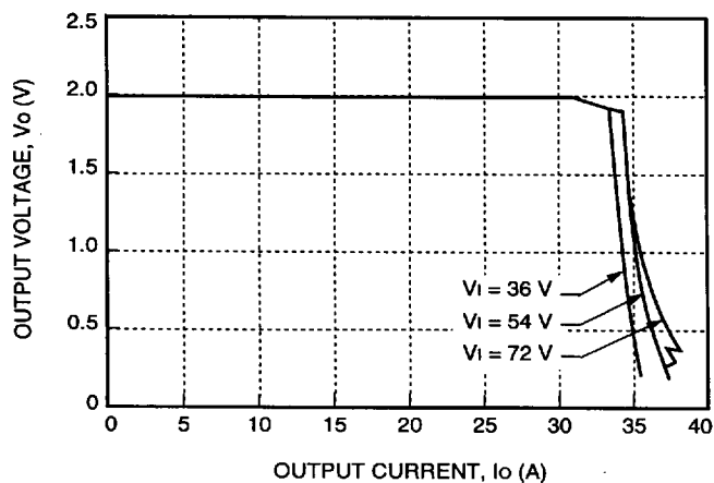
Figure 2. Typical FW150D Output Characteristics at Room Temperature
