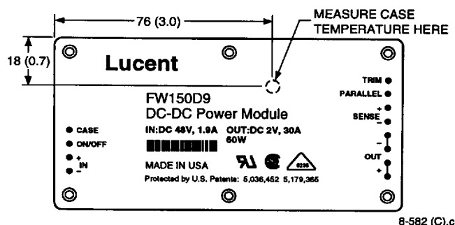
Figure 18. Case Temperature Measurement Location
