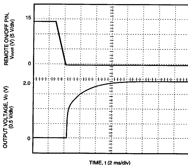
Figure 8. Typical FW150D Start-Up Transient at Room Temperature, 48 V Input, and 30 A Output
