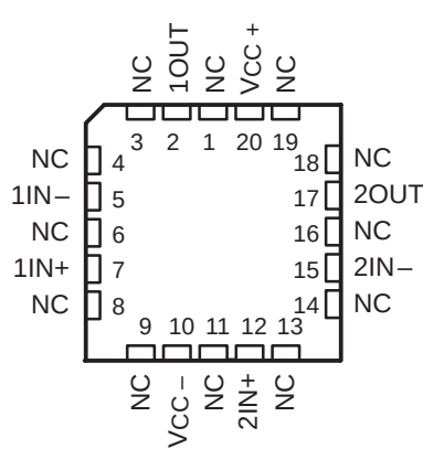
TLE2062M, TLE2062AM, TLE2062BM FK PACKAGE (TOP VIEW)
