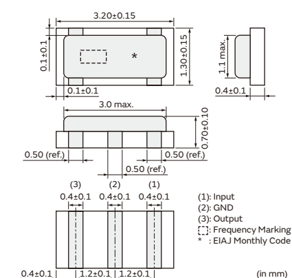
CSTNE_GH5C 8.00-13.99MHz
