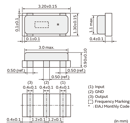
CSTNE_VH3C 14.00-20.00MHz
