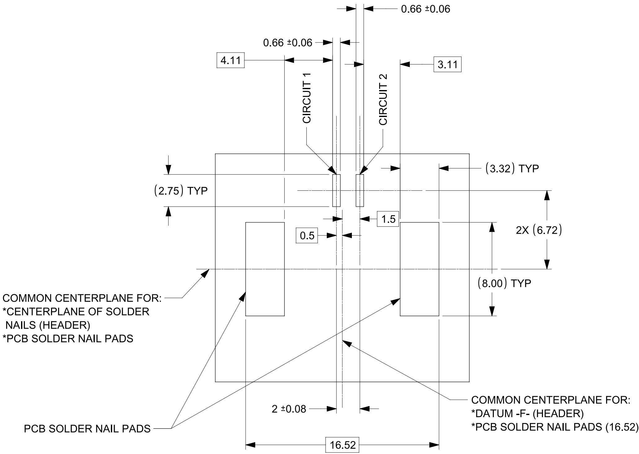
PCB LAYOUT
