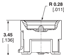
Mated Position
