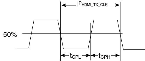
Figure 59. TMD5 Clock Signal Definitions
