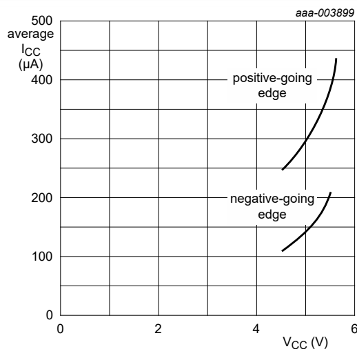
Fig. 11. Average additional supply current as a function of V_{\text{CC}} for 74HCT132; linear change of V_i between 0.1V_{\text{CC}} to 0.9V_{\text{CC}} .
