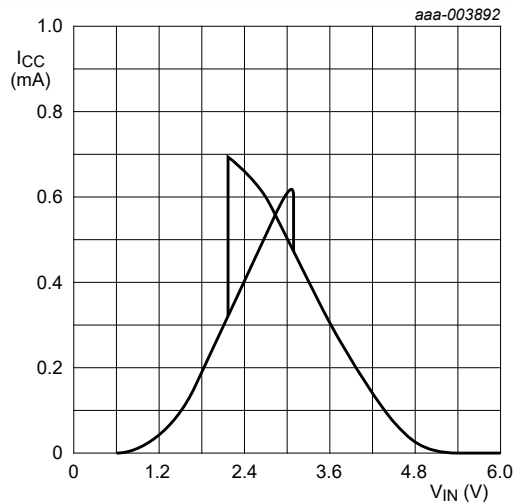
c. V_{CC} = 6.0\text{ V}
