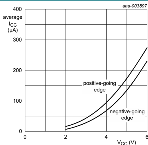
Fig. 10. Average additional supply current as a function of V_{\text{CC}} for 74HC132; linear change of V_i between 0.1V_{\text{CC}} to 0.9V_{\text{CC}} .
