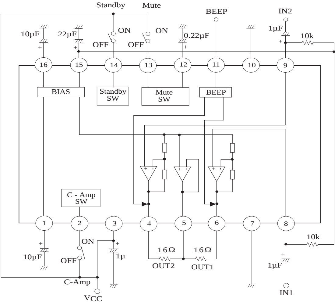
Circuit Function Block Diagram
