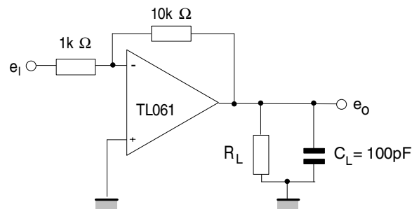
Figure 19. Gain-of-10 inverting amplifier
