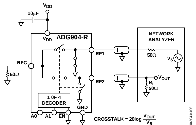
Figure 22. Crosstalk
