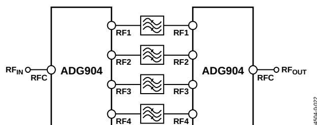
Figure 27. Filter Selection
