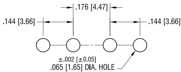
MOUNTING LAYOUT FOR TWO CLIPS
