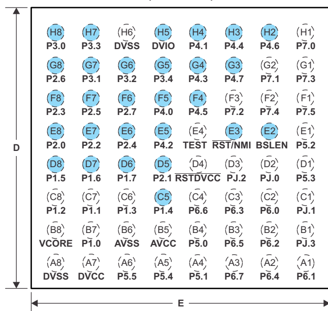
YFF PACKAGE (TOP VIEW)
