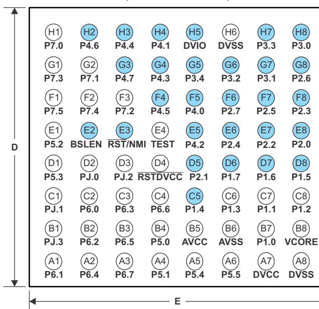
YFF PACKAGE (BALL-SIDE VIEW)
