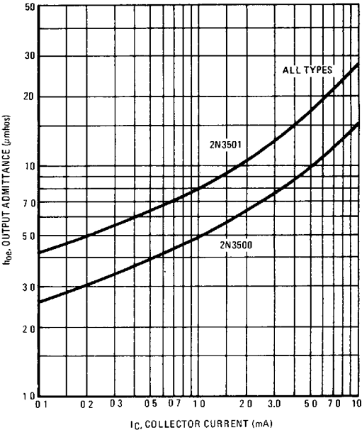
FIGURE 7 — OUTPUT IMPEDANCE
