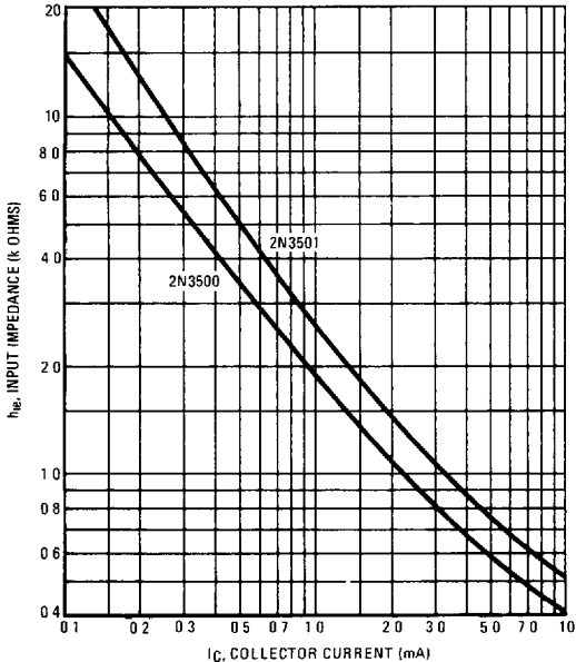
FIGURE 8 — INPUT IMPEDANCE
