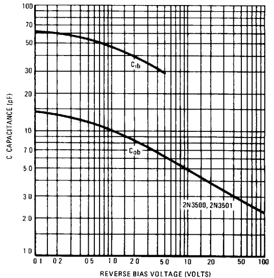
FIGURE 5 — CAPACITANCE
