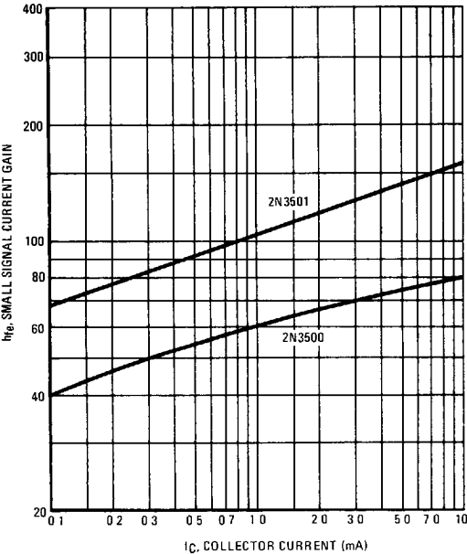
FIGURE 6 — CURRENT GAIN
