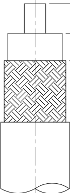
RECOMMENDED CABLE STRIPPING DIM'S
