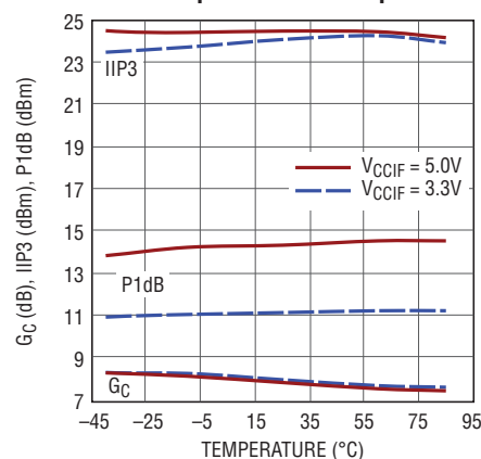
1750MHz Conversion Gain, IIP3 and RF Input P1dB vs Temperature
