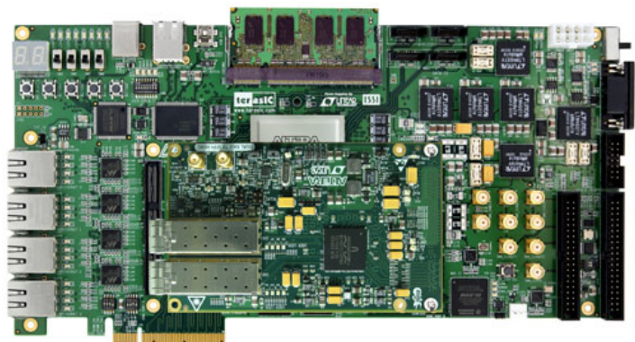
DUAL XAUI TO SFP+ HSMC BOARD connects to the Altera DE4 FPGA Development Board
