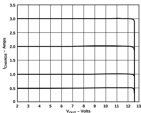
Figure 22. CCCV Characteristic with Ideal Load
