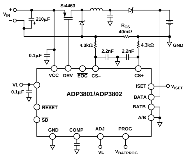
Figure 33. Low Side Current Sensing For Low Overhead Charging
