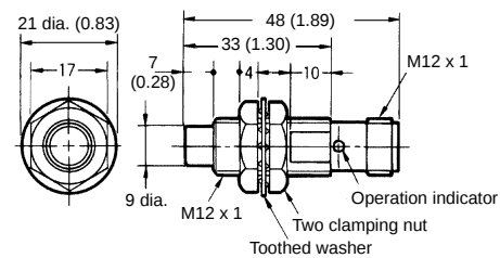
Fig.17: E2E-X10ME□-M1/F□-M1-N
