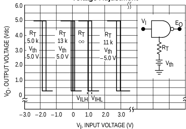
Figure 4. MC1489 Input Threshold Voltage Adjustment
