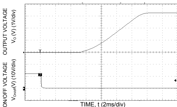
Figure 15. Typical Start-Up Using Remote On/Off with Low-ESR external capacitors ( 7 \times 150\mu\text{F} Polymer) ( V_{in} = 12.0\text{Vdc} , V_o = 3.3\text{Vdc} , I_o = 3\text{A} , C_o = 1050\mu\text{F} ).
