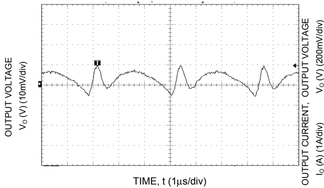
Figure 8. Typical Output Ripple and Noise ( V_{IN} = 12.0Vdc , V_O = 0.75Vdc , I_O = 3A ).
