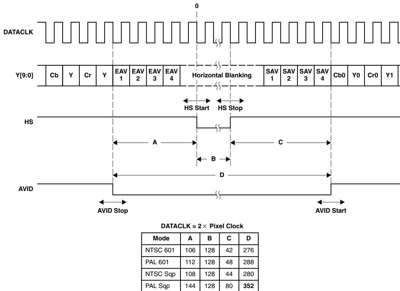
Figure 2–22. Horizontal Synchronization Signals for 10-Bit 4:2:2 Mode
