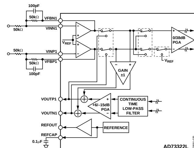
Figure 35. Analog Input (DC Coupled) Using Internal Amplifiers
