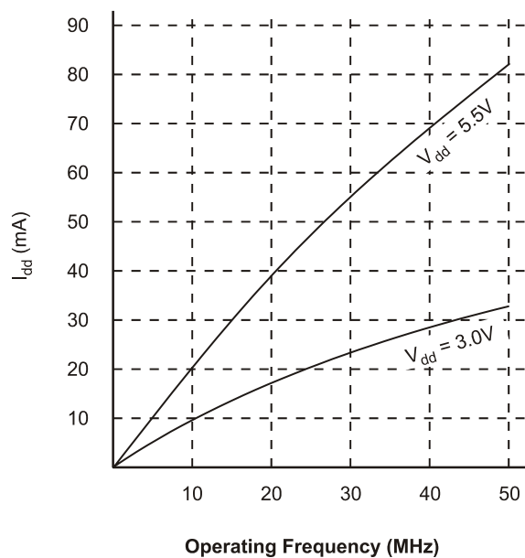
Active Supply Vs Operating Frequency (External Clock)
