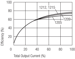
R12A/Bxx
