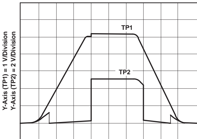
X-Axis = 0.2 ms/Division Figure 18. V_{CC} vs Output Waveform 3
