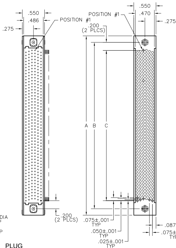
PLUG
