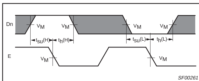
Waveform 4. Data set-up time and hold times
